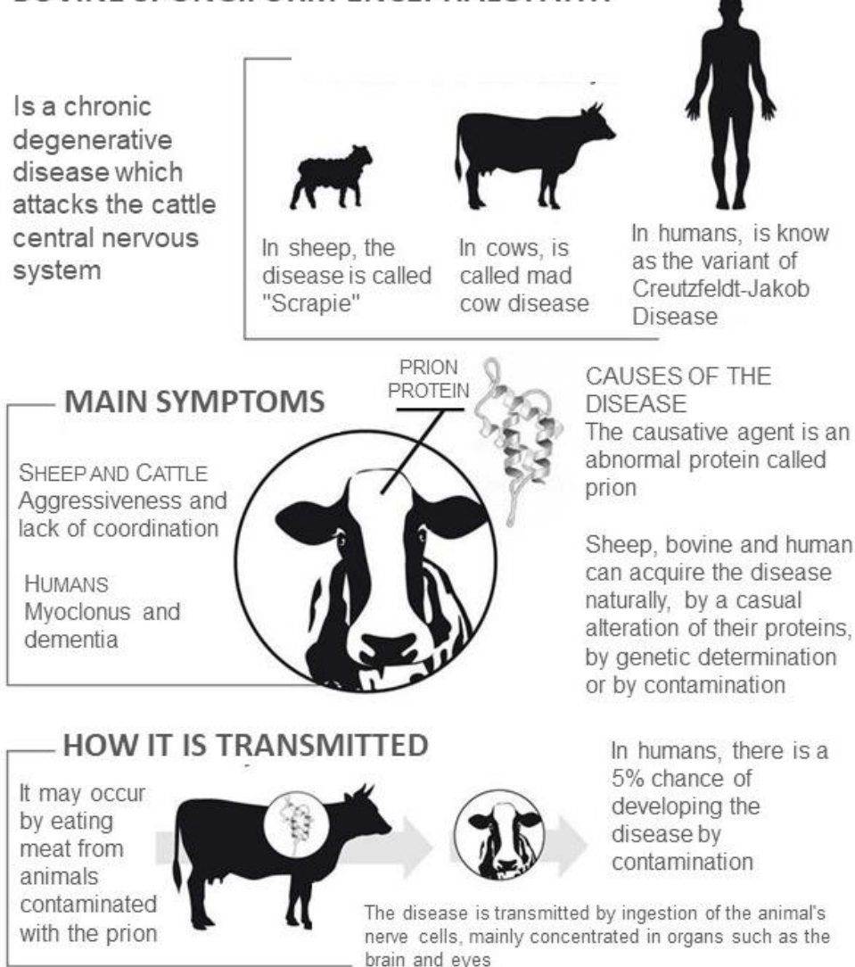
Figure 1 - Origin and transmission of Bovine Spongiform Encephalopathy (BSE). (Image adapted from: osaogoncalo.com.br/geral/21367/four-persons-are-interned-with-suspicious-of-mad-cow-disease-in-rj )
